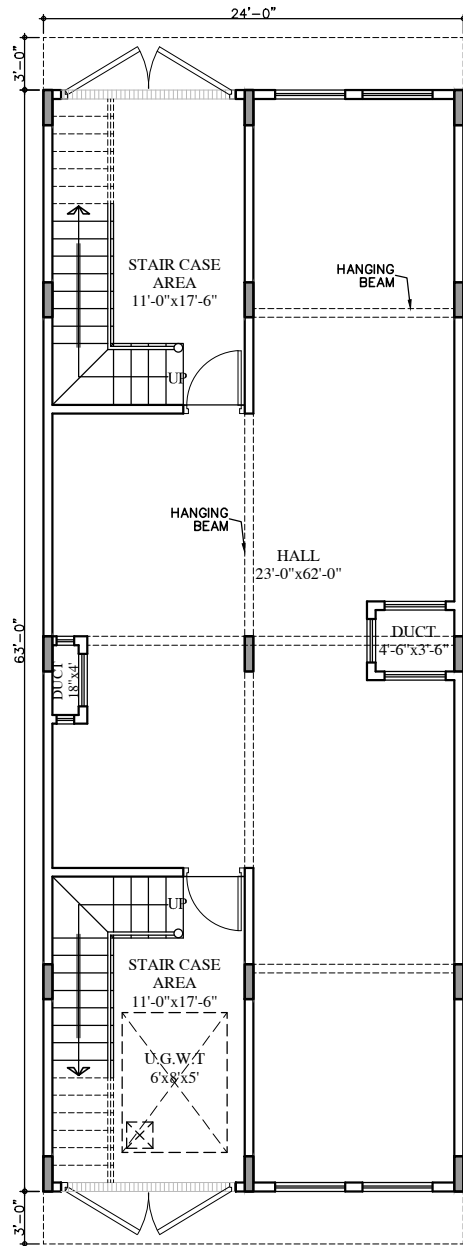
GROUND FLOOR PLAN Scale: 1'-0" = 3/32"
