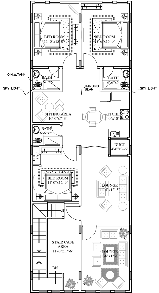
SECOND FLOOR PLAN Scale: 1'-0" = 3/32"
