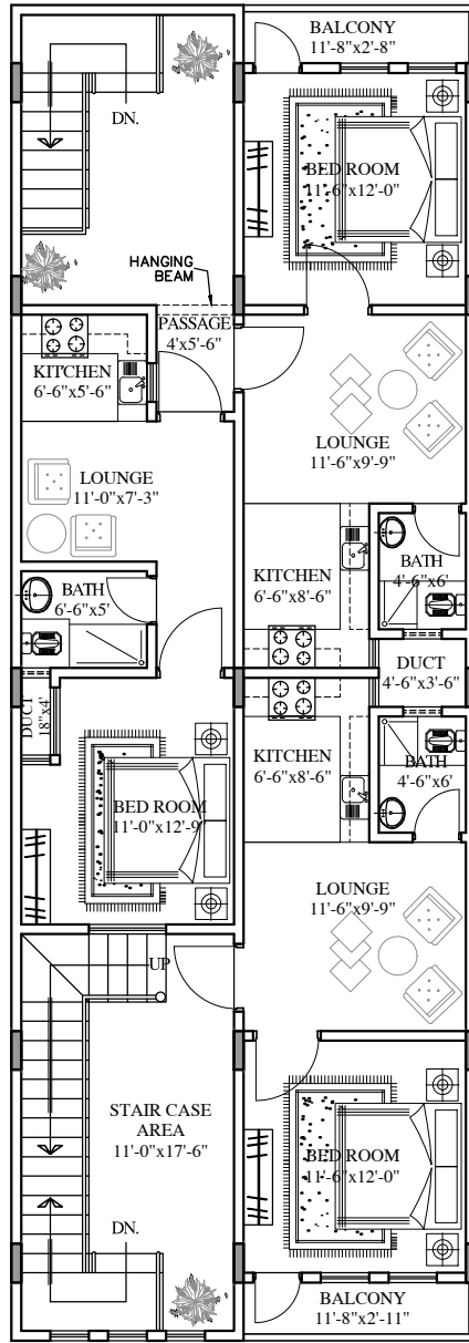
FIRST FLOOR PLAN Scale: 1'-0" = 3/32"
